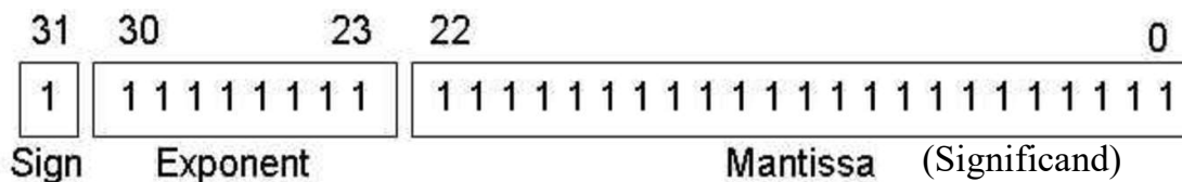
Fig 1: Floating point representation in IEEE Short Real: 32 bits
